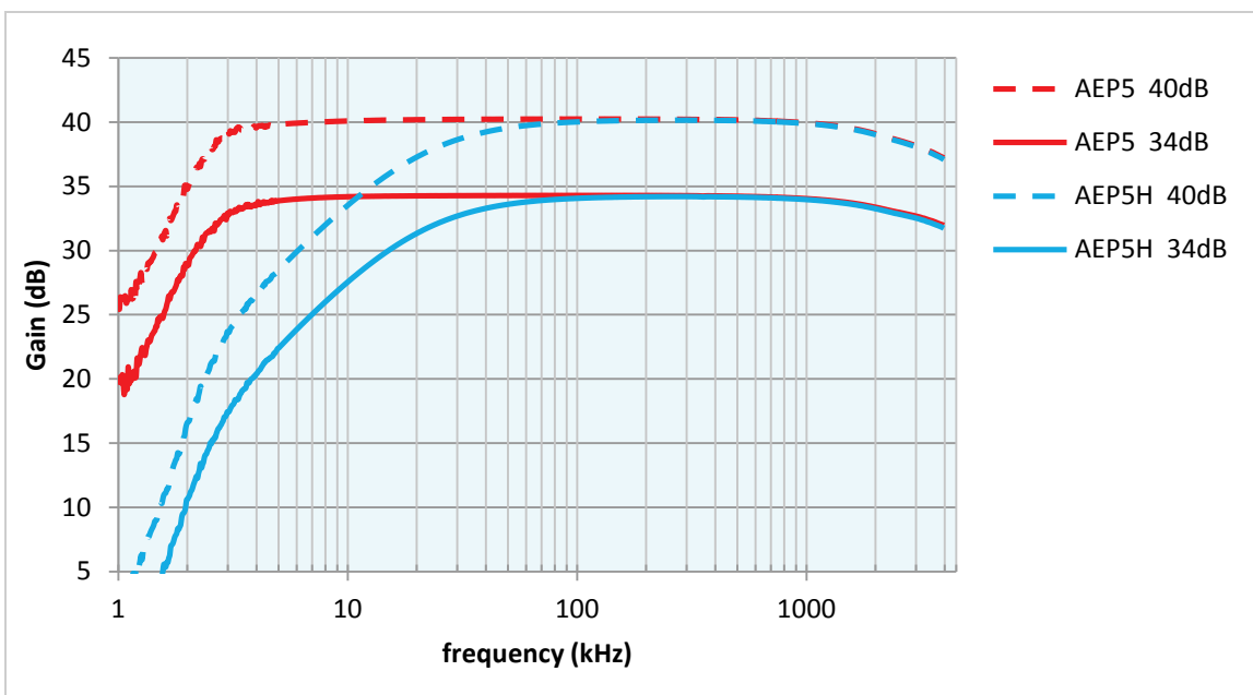
Figure 5: Frequency response of AEP5 and AEP5H preamplifier
