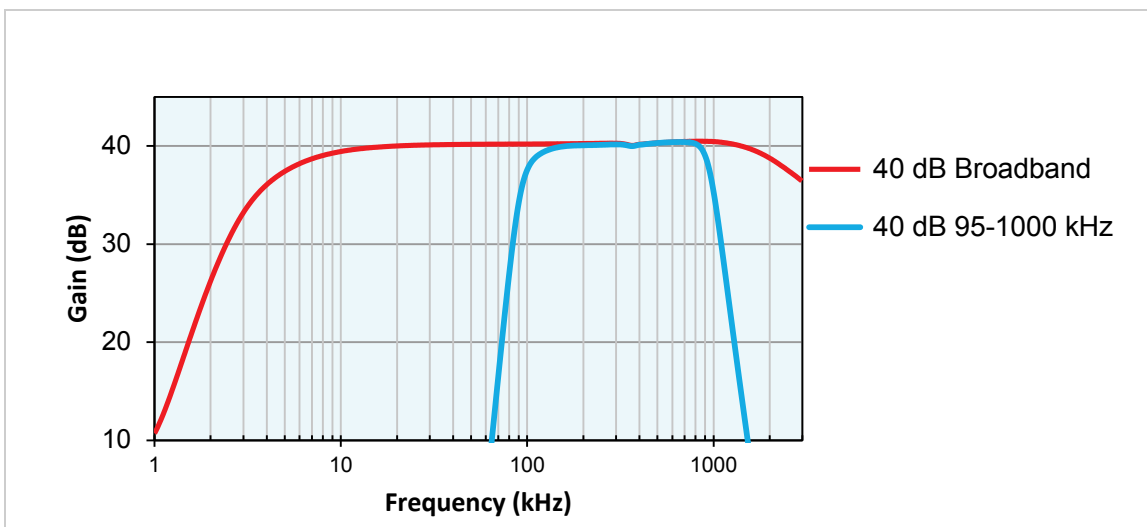
Figure 3: Frequency response of AEP3N with two different band-pass filters. “Broadband” refers to bypass-filter. Other frequency filter available, see table below.
